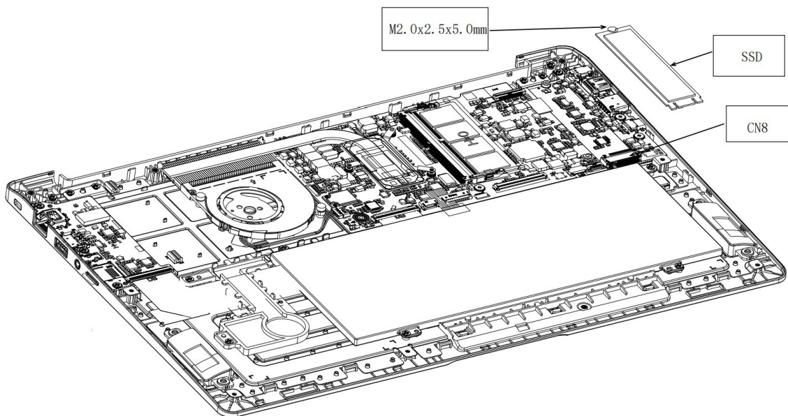
Figure 4-13 Removing SSD
