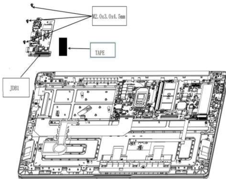
Figure 4-23 Removing IO Board
