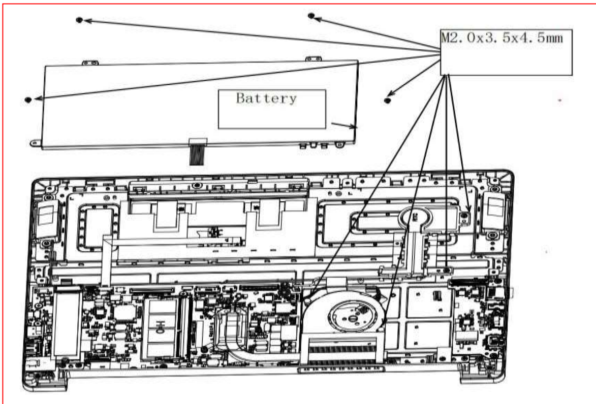
Figure 4-9 Removing battery pack
