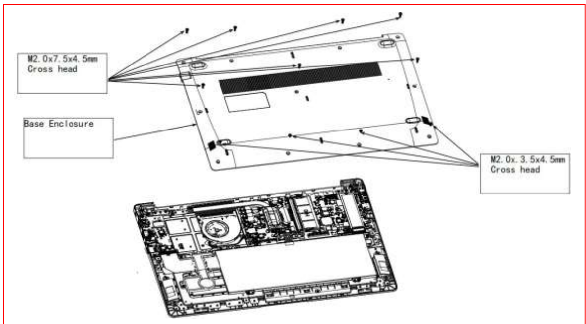
Figure 4-7 Removing Base Enclosure
