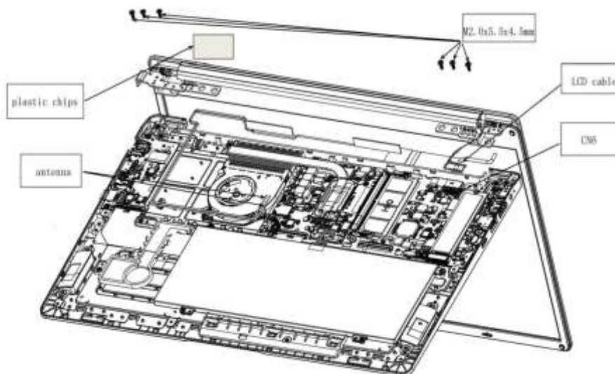
Figure 4-17 Removing the LCD Module assembly
