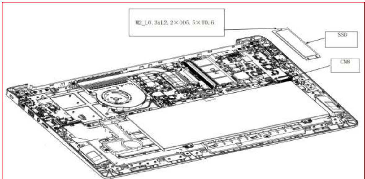
Figure 4-13 Removing SSD
