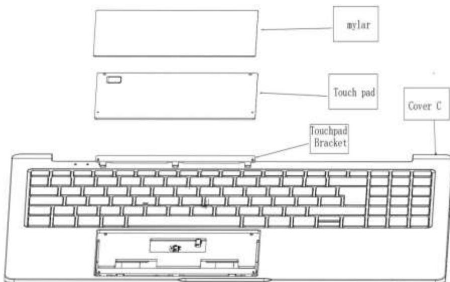
Figure 4-35 Removing Touch pad
