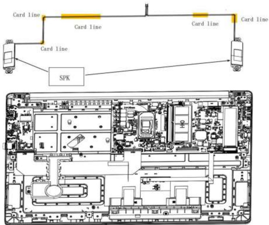
Figure 4-25 Removing Speaker
