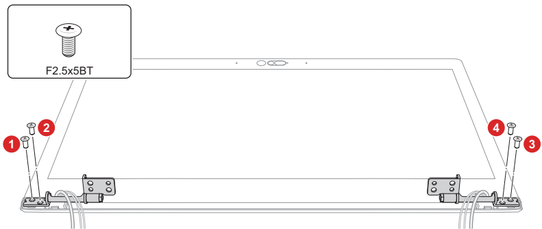
Figure 4-56 Installing the LCD unit (3)
