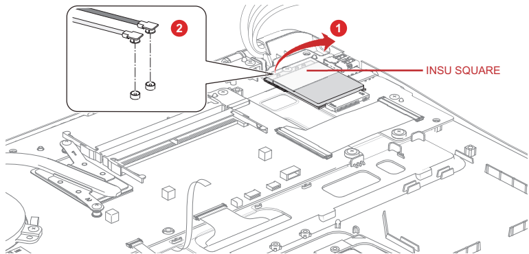
Figure 4-21 Removing the 3G module (1)
