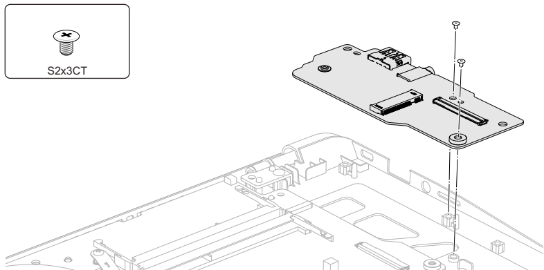
Figure 4-24 Removing the USB board (2)
