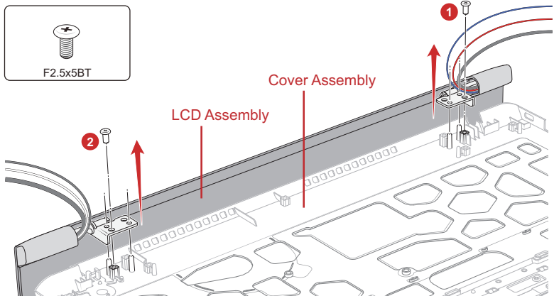
Figure 4-49 Removing the LCD unit (1)
