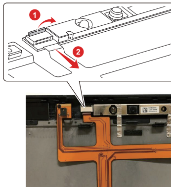
Figure 4-60 Removing the camera module (4)
