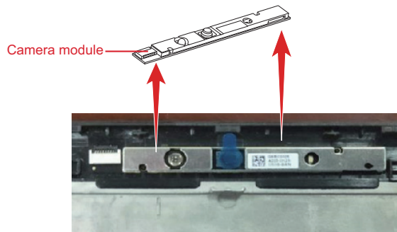
Figure 4-60 Removing the camera module (4)
