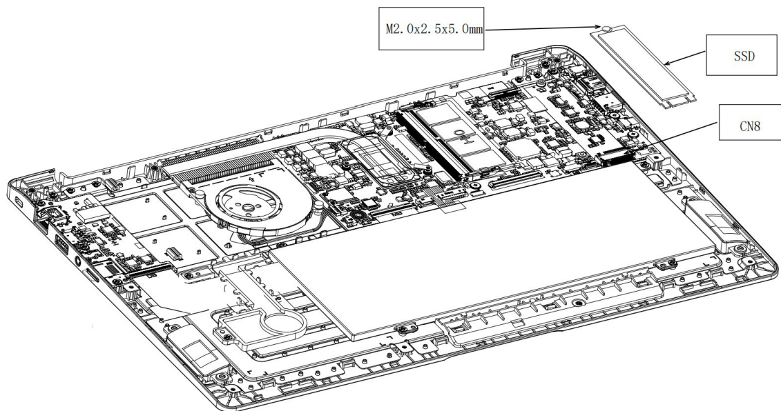
Figure 4-13 Removing SSD
