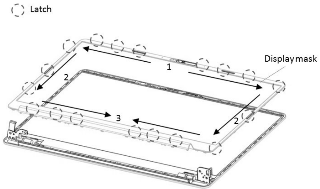
Figure 4-28 Removing the LCD Module Mask
